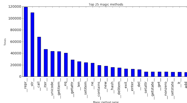
Figure 3: Most common magic methods ( __init__ not included).
